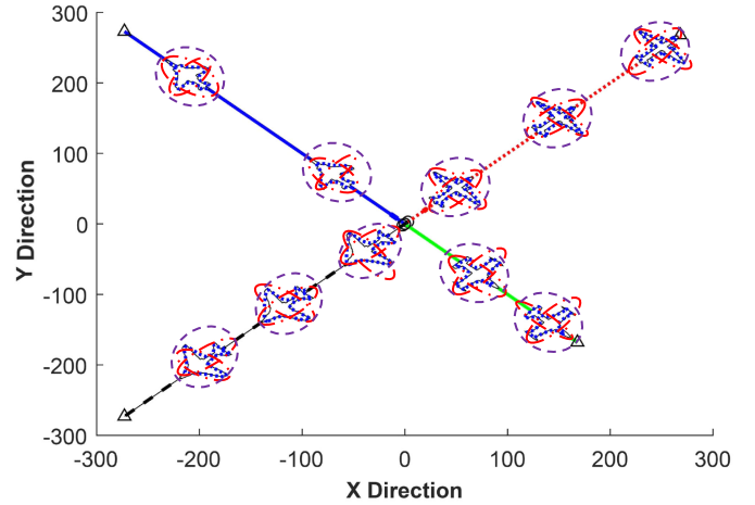
Fig. 4. Scenario I. True target trajectories (the straight lines) in the x - y plane with start/end ( \circ/\Delta ). The true target shape is shown in black line, our B-spline method in blue-dotted line, the multi-sub-object method in red-dash-dotted line and the random matrix method in purple-dashed line. All four targets start from the origin. The target plots shown are at intervals of 20 time steps.
