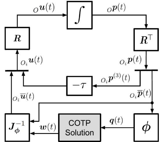
Fig. 2. A block diagram representing Algorithm 1. Bold letters indicate the vectors in which the relative values of the individual agents are contained (e.g., q(t) = [q_1(t)^\top, q_2(t)^\top, \dots, q_N(t)^\top]^\top ).
