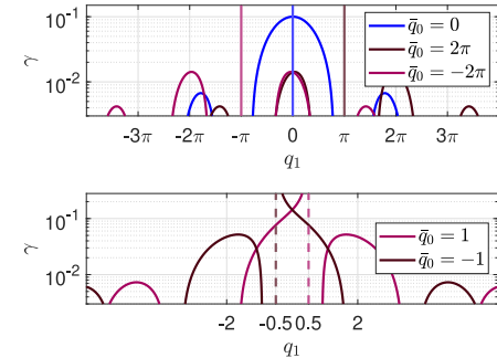
Fig. 7. Zero-dynamics equilibria for intermediate values of \gamma and various desired tip orientations \bar{q}_0 . Equilibria are found intersecting \xi = \Gamma_2(\bar{q}_0, q_1)/(6\bar{q}_0 - 12q_1) and \xi = \gamma . The upper plot reports the graphs for \bar{q}_0 \in \{-2\pi, 0, 2\pi\} and the lower one for \bar{q}_0 \in \{1, -1\} .
