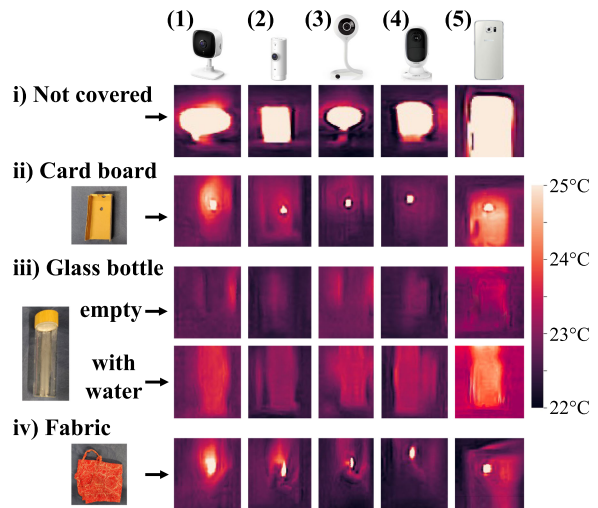
FIGURE 3. Thermal fingerprint of hidden cameras with different materials. Cameras: (1) TP-Link Tapo C100, (2) D-Link DCS-8000LH, (3) Nedis WIFICI11CWT, (4) Reolink Argus 2, and (5) Samsung Galaxy S6.
