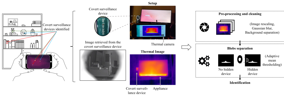
FIGURE 1. Thermal imaging targeting a covert surveillance device in a living room and ambient light conditions, and the processing pipeline for recognizing covert surveillance devices from thermal camera input.
