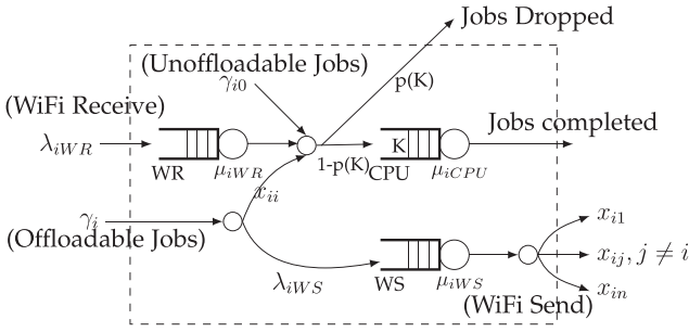
Fig. 4. A sensor node modelled as network of queues. CPU, WR, and WS represent CPU, WiFi Receiver, and WiFi Sender queues, respectively.
