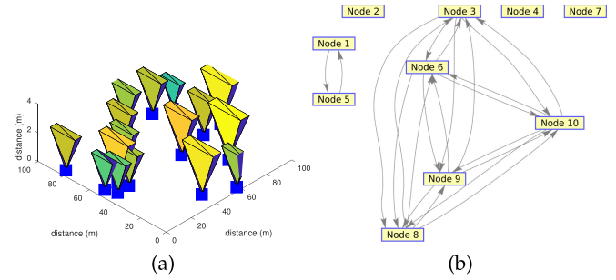
Fig. 7. Simulation setup for one monte-carlo simulation. (a) Ten sensors (blue squares) with uneven FOV placed randomly on the simulation platform of 100m \times 100m size. (b) Visualizing sensor connectivity based on spatial positioning.
