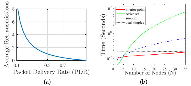
Fig. 5. (a) Average no. of retransmissions required due to imperfect channel. (b) Time complexity of various linear solvers.
