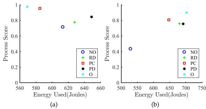
Fig. 12. Efficiency Scores: (a) RWP and (b) SAIVT.
