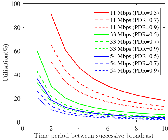
Fig. 6. Queue utilization of server in proactive setting under various network conditions (Lower is better). Data size set at 1 Mb.
