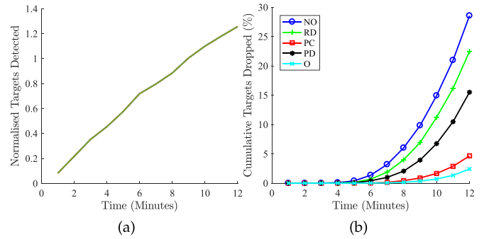
Fig. 10. Simulation results for RWP target data with Bandwidth 11 Mbps NSI exchange frequency of 5 seconds and range of communication limited to 60 meters. (a) Normalized Target arrival rate per nodes over simulation time (b) Targets dropped over Arrival Rate. NO dropped the most (30 percent of all targets). Centralized algorithms performed best with at least 80 percent reduction in dropped targets and distributed algorithms perform in between.
