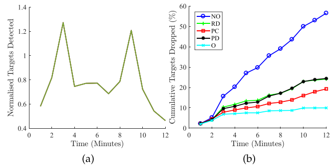
Fig. 11. Simulation results for SAIVT target data with Bandwidth 11 mbps NSI exchange frequency of 5 seconds and range of communication limited to 60 meters. (a) Normalized Target arrival rate per nodes over simulation time. (b) Cumulative targets dropped over time. Proposed algorithms perform significantly better than the NO case. Distributed algorithms dropped less than half of the baseline and the Oracle dropped only about sixth.
