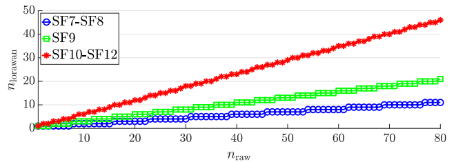
Fig. 13. Number of JSON-encoded LoRaWAN packets as a function of the number of raw packets to be sent, for various values of the SF.
