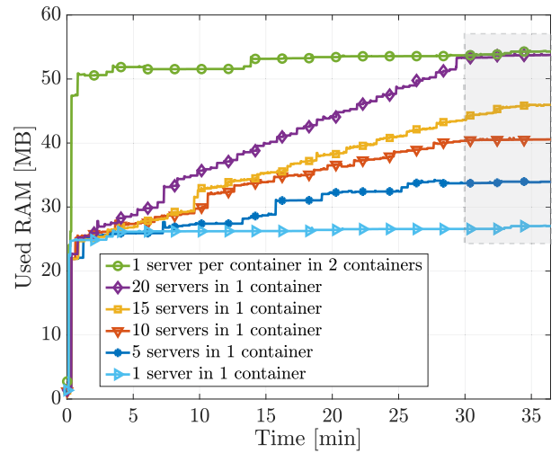
Fig. 10. Experimental comparison between RAM memory occupation (on an ASUS laptop with i7 CPU) with “parallel container” and “parallel vEN” virtualization approaches.
