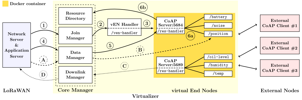
Fig. 5. Building blocks and interactions of the virtualization architecture following the “parallel vEN” approach.
