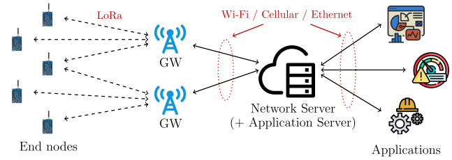
Fig. 1. General LoRaWAN architecture providing IoT-oriented information to external applications.
