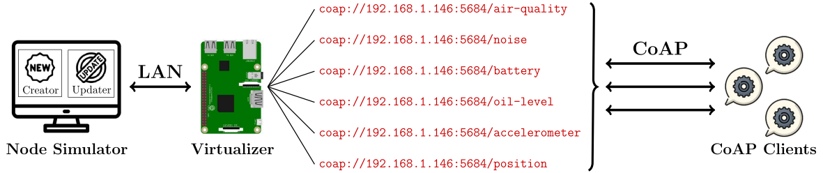
Fig. 7. Setup for the experimental evaluation of the proposed virtualization architecture, with the Virtualizer hosted on a RPi3. The experimental performance evaluation has also been carried out hosting the Virtualizer on a laptop.
