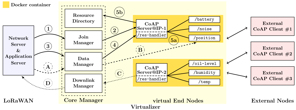
Fig. 4. Building blocks and interactions of the virtualization architecture following the “parallel container” approach.
