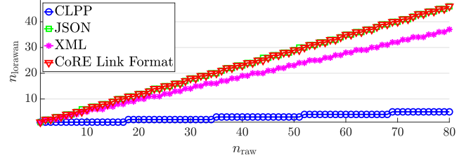
Fig. 18. Number of LoRaWAN packets as a function of the number of raw packets to be sent adopting a LoRaWAN SF equal to SF10-SF12 (sharing the same maximum payload length \ell_{\text{SF10}} = \ell_{\text{SF11}} = \ell_{\text{SF12}} = 51 bytes), shown for each considered data representation format.
