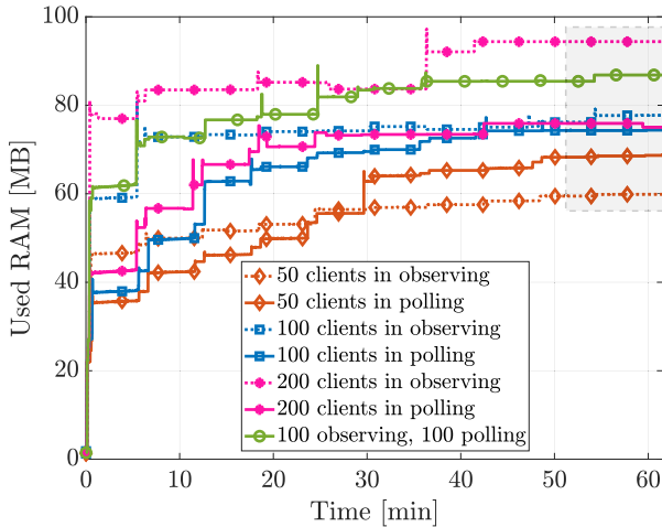
Fig. 9. Experimental RAM utilization comparison (on an ASUS laptop with i7 CPU), splitting the CoAP clients in observing and polling .
