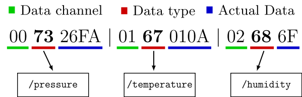
Fig. 2. Example of received CLPP-encoded uplink packet, with corresponding CoAP resources (as detailed in Section IV).
