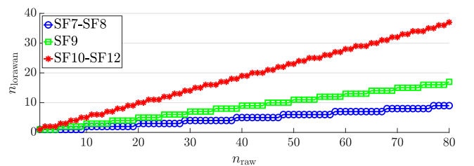
Fig. 14. Number of XML-encoded LoRaWAN packets as a function of the number of raw packets to be sent, for various values of the SF.
