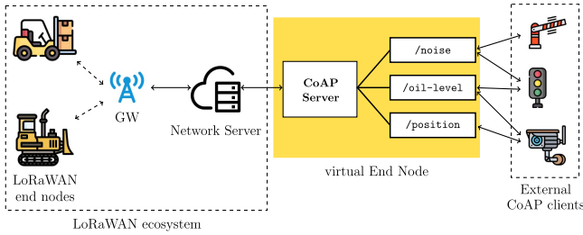
Fig. 3. LoRaWAN architecture extended with the Virtualizer.
