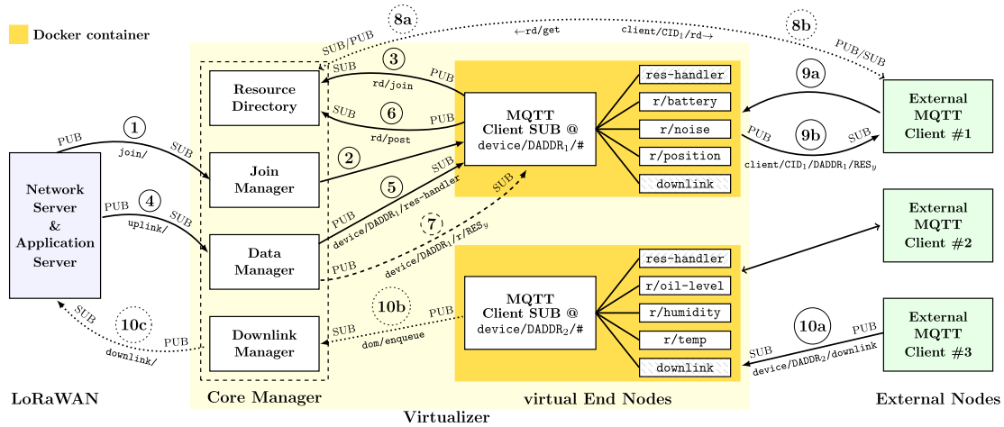
Fig. 6. Building blocks and interactions of the virtualization architecture following the “parallel container” approach, but only featuring MQTT as data exchange protocol.
