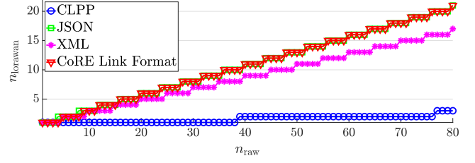
Fig. 17. Number of LoRaWAN packets as a function of the number of raw packets to be sent adopting a LoRaWAN SF9 (having a maximum payload length \ell_{\text{SF9}} = 115 bytes), shown for each considered data representation format.
