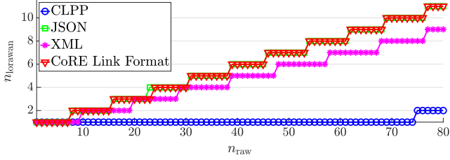
Fig. 16. Number of LoRaWAN packets as a function of the number of raw packets to be sent adopting a LoRaWAN SF equal to SF7-SF8 (sharing the same maximum payload length \ell_{SF7} = \ell_{SF8} = 222 bytes), shown for each considered data representation format.
