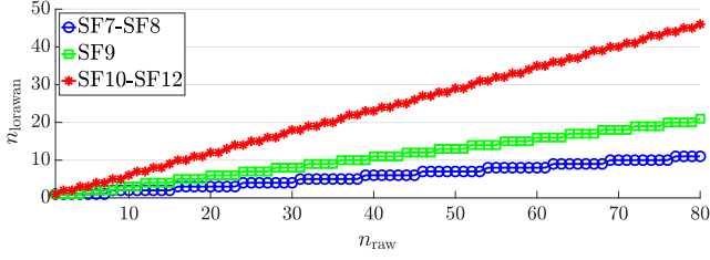
Fig. 15. Number of CoRE Link Format-encoded LoRaWAN packets as a function of the number of raw packets to be sent, for various values of the SF.
