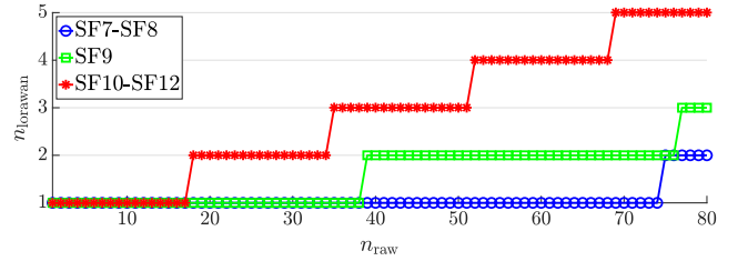
Fig. 12. Number of CLPP-encoded LoRaWAN packets as a function of the number of raw packets to be sent, for various values of the SF.
