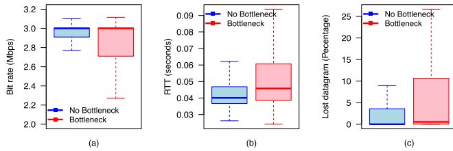
Fig. 1. Impact of network bottleneck on performance degradation at UE.
