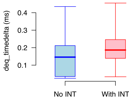
Fig. 7. Impact on queuing delay of data packets when a virtual P4 switch performs in-band network telemetry in a mobile network.
