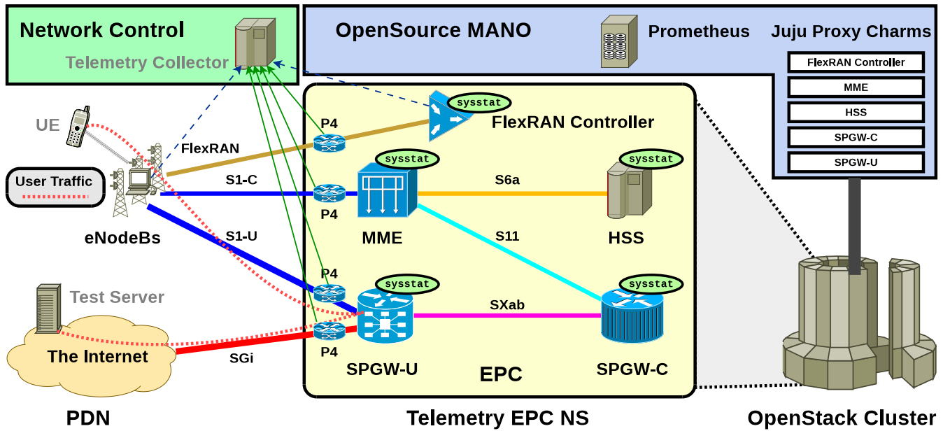
Fig. 2. Testbed Infrastructure of the Cloudified Mobile Network.
