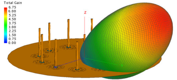
Fig. 2. ESPAR antenna's radiation pattern for one of its directional main beam configurations. The radiation pattern corresponds to the steering vector V_{\max}^1 = [1, 1, 1, 1, 1, 0, 0, 0, 0, 0, 0, 0] and is provided by opening five neighboring passive elements, which are directors, while the others are reflectors shortened to the antenna ground (see text for explanations).
