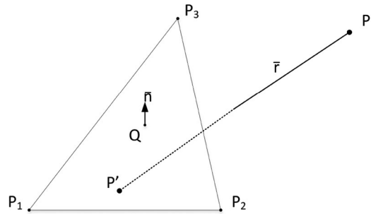
Fig. 3. Raycasting and triangle intersections.
