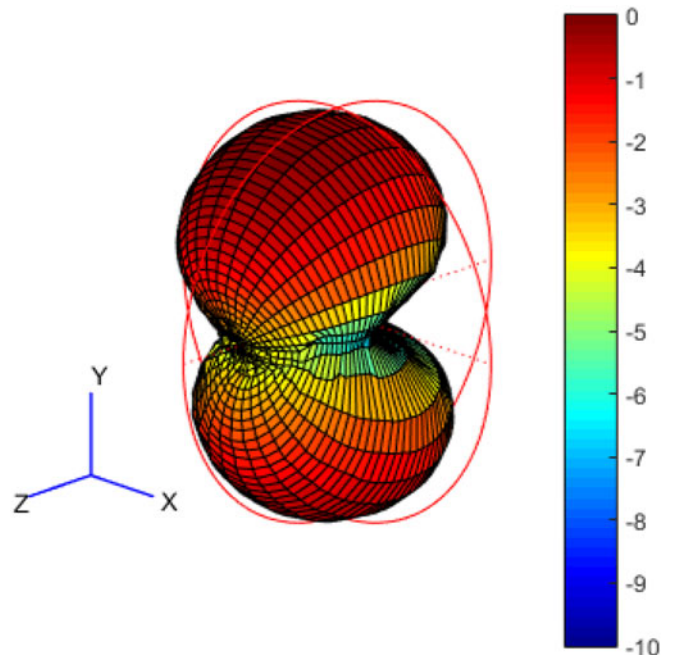
Fig. 7. Conformal aperture relative gain pattern (relative to maximum of 41.7 dBi).
