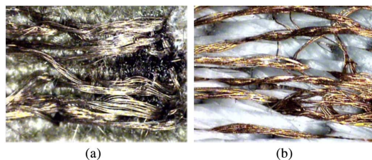
Fig. 5. Microscope images: (a) copper wire; (b) copper wire with Teflon.
