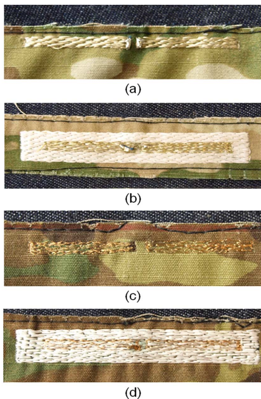
Fig. 3. Embroidered dipoles: (a) Amberstrand, (b) Amberstrand on Teflon, (c) copper yarn, and (d) copper yarn on Teflon.
