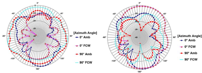
Fig. 6. Measured ( left ) E-Phi polarization gain (dBi) [elevation plane] and ( right ) E-Theta polarization gain [elevation plane] for Amberstrand and 7-stranded copper yarn (fcw). Dipole is horizontal in the plane of the paper.
