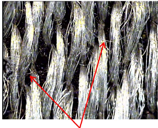
Fig. 2. Example of the filamenting of the Amberstrand thread seen under a microscope. Note the fine filaments running normal to the embroidered yarn.
