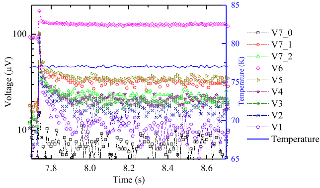
Fig. 8. All strand voltages at 440 A (Strand 8-15 voltages are below 10 \mu\text{V} ).
