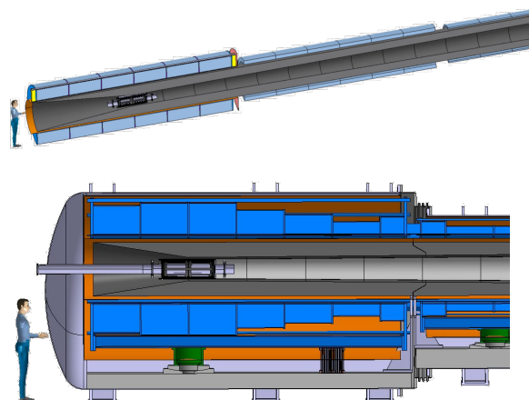
Fig. 2. Schematic view of the HTS target, decay and capture channel proposed (top), with a detail of the high field solenoids around the proton target area (bottom).
