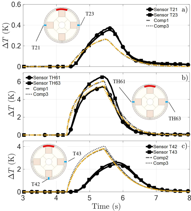
Fig. 5. Temperature time evolution for simulation performed with \Gamma_1 and \Gamma_2 . (a) Upstream of the heated region, (b) in the heated region, and (c) downstream of the heated region. Gray lines \Gamma_1 , yellow lines \Gamma_2 . In the insets the location of the temperature sensors is shown, while the red arches identify the heated component (Comp1 = AO_{15,3} ; Comp2 = AO_{17,5} ; Comp3 = AO_{19,7} ).
