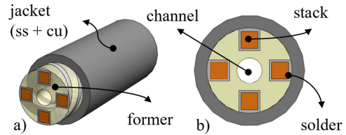
Fig. 1. (a) 3D CAD drawing of the VIPER cable and (b) 2D CAD cross-section of the VIPER cable. The main components labels are also displayed.
