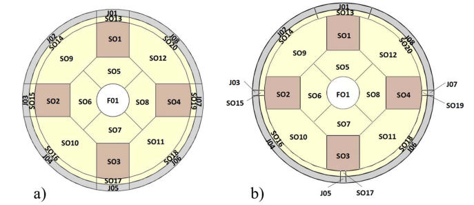
Fig. 3. Cross-section discretization and naming scheme associated to \Gamma_1 (a) and \Gamma_2 (b).
