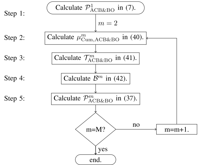
Fig. 4. Flowchart for deriving the RA success probability in the M th time slot with the ACB&BO scheme \mathcal{P}_{ACB\&BO}^M .
