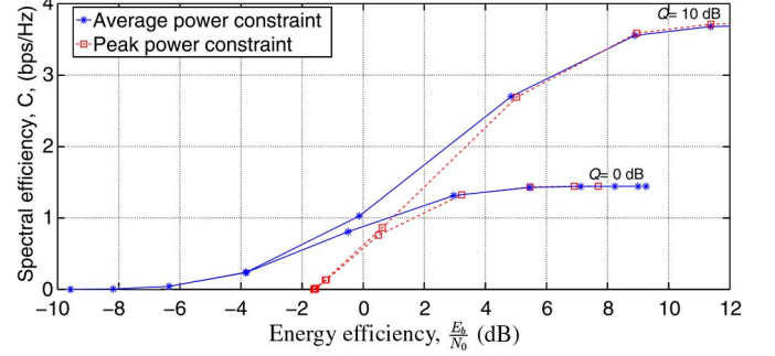
Fig. 2. Per-link spectral-energy efficiency trade-off for CR channel with average and peak power constraints (Rician factor K = 5 ).
