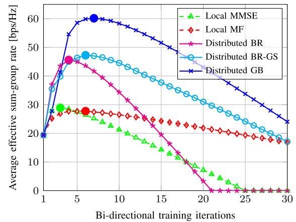
Fig. 4. Average effective sum-group rate versus number of bi-directional training iterations, with r_t = 1000 .
