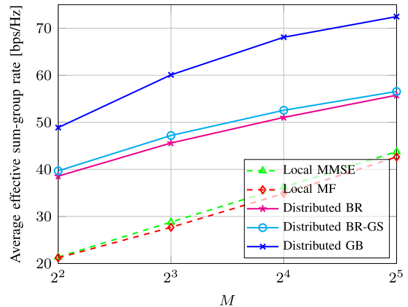
Fig. 7. Average effective sum-group rate versus number of antennas at each BS, with r_t = 1000 .
