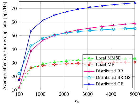
Fig. 5. Average effective sum-group rate versus resource block size.
