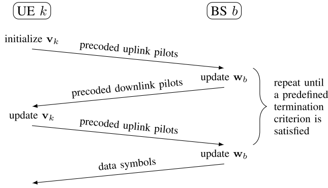
Fig. 1. Schematic representation of iterative bi-directional training in a single-UE, single-BS setting. To transmit the precoded uplink pilots, UE k uses \mathbf{v}_k as precoder.
