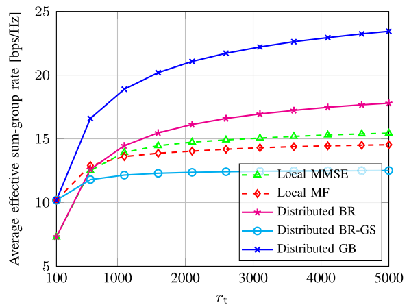
Fig. 8. Average effective sum-group rate versus resource block size at low SNR ( \sigma_{\text{BS}}^2 = \sigma_{\text{UE}}^2 = -75 dBm).
