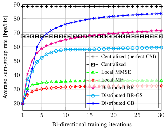
Fig. 3. Average sum-group rate versus number of bi-directional training iterations.
