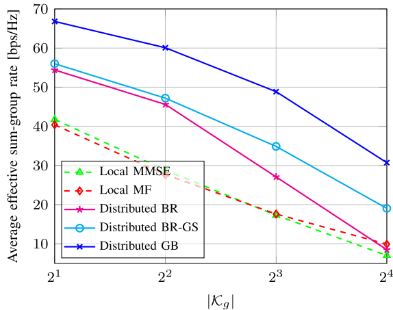
Fig. 6. Average effective sum-group rate versus number of UEs in each multicast group, with r_t = 1000 .
