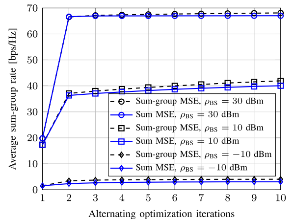
Fig. 2. Average sum-group rate resulting from the sum-group MSE minimization and the sum MSE minimization versus number of alternating optimization iterations for different values of \rho_{\text{BS}} .
