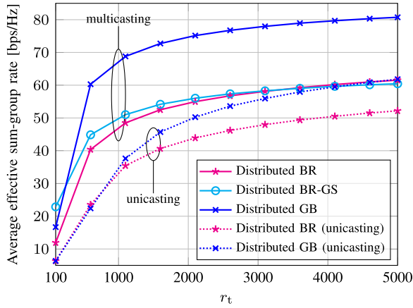
Fig. 9. Average effective sum-group rate versus resource block size in comparison with the unicast precoding design [20] with the same CSI accuracy.
