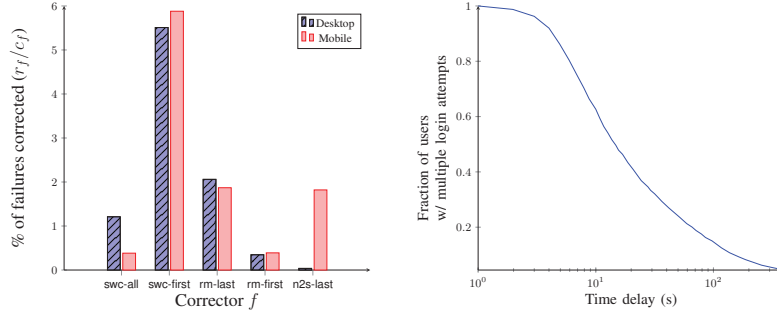
Fig. 3: (Left) The fraction of failed logins correctable by \mathcal{C}_{top5} in a 24-hour study at Dropbox. (Middle) Performance of \mathcal{C}_{top5} on mobile versus desktop. For each corrector in \mathcal{C}_{top5} we plot the fraction of failures for each platform correctable by the corrector. (Right) CDF of time delay (in seconds) between the first failed login due to a typo and first successful login. Included are only users that had a failed login attempt and later a successful one.
