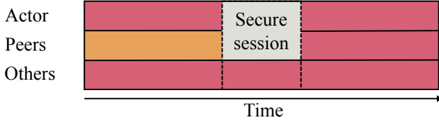
(a) Adversary model with PCS through limited compromise We denote with the orange box (the left side of the “peers” row) a limited form of compromise, which allows the adversary some extra power without revealing the long-term key.
