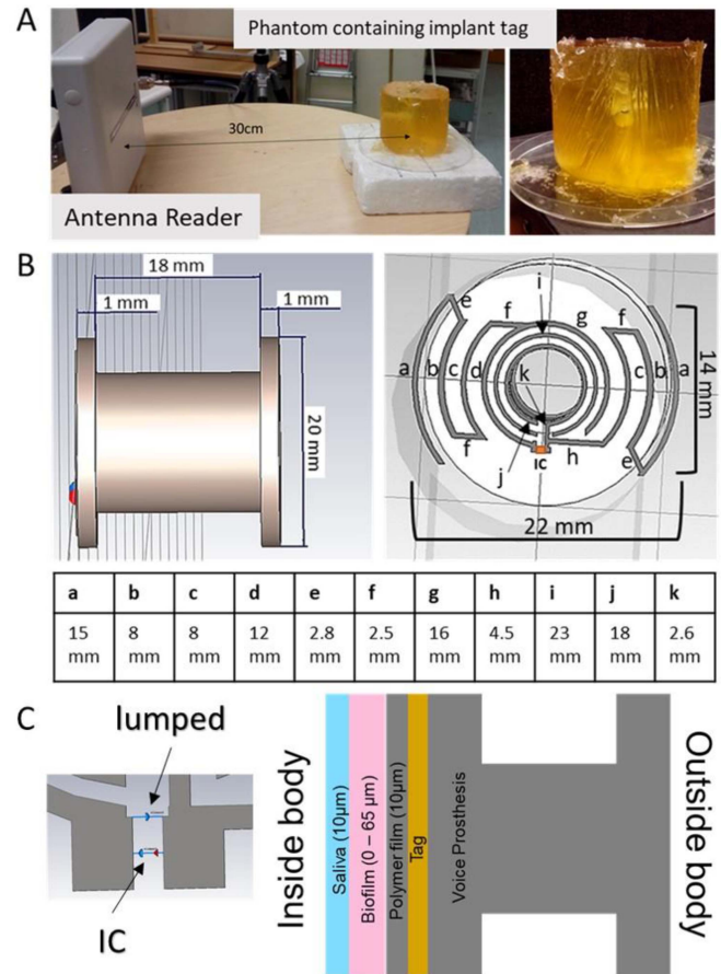
Fig. 1. UHF RFID voice prosthesis sensor design implanted within a neck phantom. A) The reader antenna calibration with a 30 cm separation between the sensor and antenna within the neck phantom (salt and gelatine); and B) The tag and sensor dimension upon the voice prosthesis model utilised for data collection. C) Exhibits the lumped element placement and IC location as well as the sketched view of the represented layers involved in the device simulation. The same neck phantom dimensions were utilized within the CST simulations and TagformancePro measurements.
