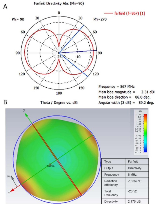
Fig. 4. Antenna directivity of a voice prosthesis mounted UHF RFID convoluted antenna sensor within a gelatine phantom. A) The polar plot showed a 2.31 main lobe magnitude visualized with a phi 90° cut. B) The total efficiency and antenna directivity shown in a 3D model view.
