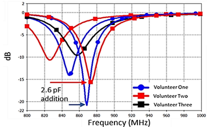
Fig. 5. Wider dielectric range effect on presented design matching based on Table II volunteer data utilized within the simulated body phantom. With a decrease in the dielectric properties from the measured gelatine phantom, only volunteer three did not require a capacitive adjustment to remain within the EU frequency at resonance. For functioning with the UHF EU frequency band, volunteer one and two required a 2.6 pF shunt to adjust the resonant frequency (red and blue, respectively).
