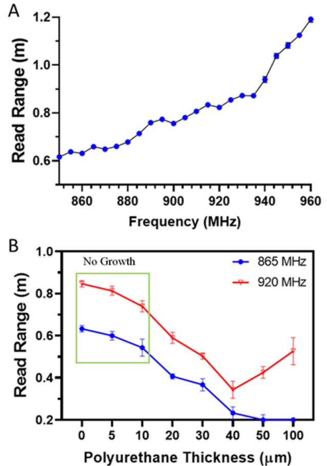
Fig. 3. Measurement of sensor function mounted on voice prosthesis within a salt and gelatine neck phantom. A) Antenna measurement over both the EU and USA UHF frequency bands without any biofilm growth adjustments (0 \mu\text{m} polyurethane thickness). B) Sensor function at both the EU (865 MHz) and USA (920 MHz) UHF frequency bands with biofilm growth adjustment to mimic C. albicans growth overtime on the voice prosthesis.
