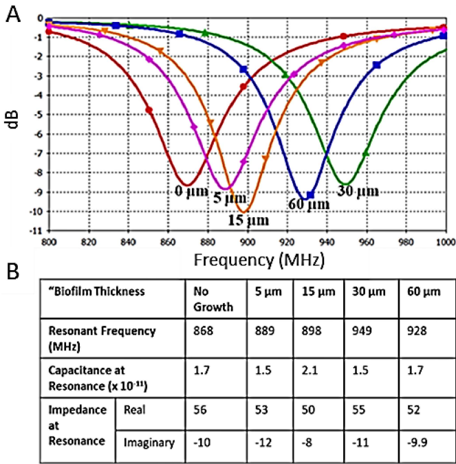
Fig. 2. S11 simulated C. albicans biofilm growth on the A) antenna sensor and b) simulated matching parameter changes due to increase in biofilm thickness. Till a mature biofilm layer is reached (30 \mu\text{m} thickness), there is a noticeable resonant frequency increase. Once the mature layer thickness doubles in height at the top of the sensor, there is a reversal in resonant frequency likely due to the saliva decoupling.
