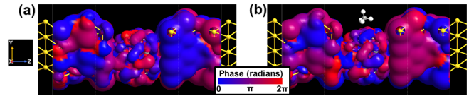
Fig. 6. (a) TE 1 of the main TS peak within the BW at 1.4 V. (b) TE 1 in the presence of CH 4 , the isovalue is 0.07.
