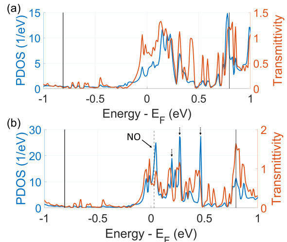
Fig. 3. Equilibrium PDOS (blue) onto the (a) C_{60} molecular channel and (b) C_{60} + NO when present NO, and relative TS (orange); the solid vertical black lines are the isolated C_{60} energy level (at left side degeneracy occurs), the dashed vertical lines are the isolated NO molecule energy level in the considered energy range.
