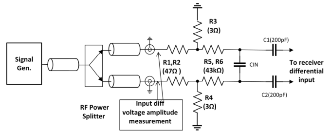
Fig. 12. Configuration for measurement of the frequency response.
