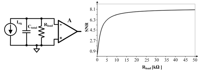
Fig. 4. A high-impedance receiver and its SNR as a function of the load resistance, i_{s,pr} = 10 nA ( M = 10 ), C_{total} = 3.5 pF, \Delta t_{pulse} = 10 ns. Only the thermal noise of R_{load} is considered.
