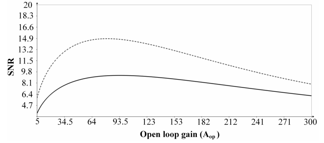
Fig. 6. SNR as a function of the preamplifier open loop gain; dotted curve: without signal shot noise, solid curve: signal shot noise included.
