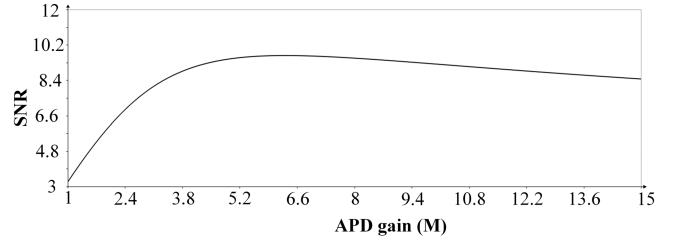
Fig. 7. SNR as a function of the APD gain M ( A_{OP} set to 80).
