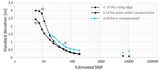
Fig. 20. The dependence of the timing jitter on the measured signal strength for three different timing detection techniques a) detection on the rising edge only, b) detection on the rising edge and pulse width based walk error compensation, c) detection on the rising and rise time measurement based timing walk error compensation.
