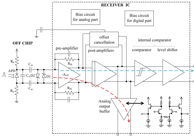
Fig. 8. Block diagram of the laser radar receiver circuit.
