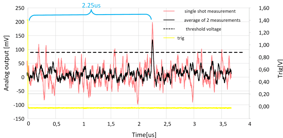
Fig. 22. Measured signal strength from the wall of a building at a distance of \sim 330\text{m} . A 1550nm laser pulse with a width of 20ns and peak power of \sim 4\text{W} and a receiver aperture of 20mm were used in the measurements.
