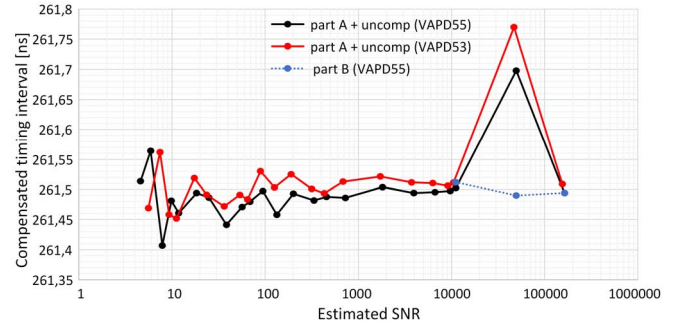
Fig. 19. Residual timing walk error. Continuous red and black lines: compensated is based on the part A of the compensation curve; blue dashed line: compensated timing results for signal levels \text{SNR} > 10\ 000 using part B of the compensation curve.
