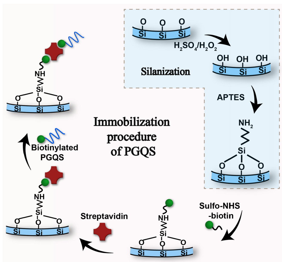
Schematic illustration of PGQS immobilization procedure (vol. 20, no. 21, see page 12560).
