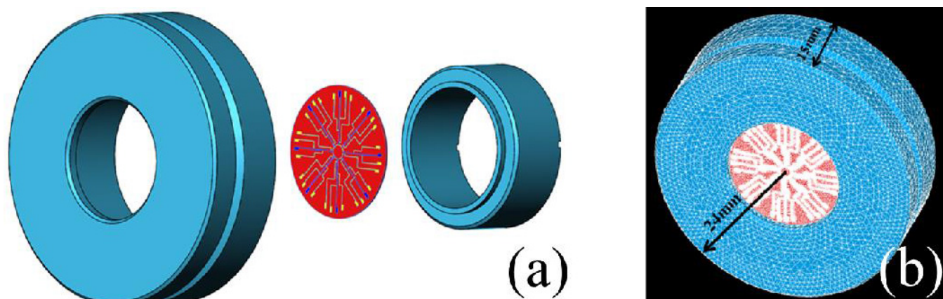
Illustration of the combined sensor and fixture structure. The blue fixture is made of copper and the red disk is the sensor (a) showing the anatomical structure and (b) the finite element mesh model. (Vol. 20, No. 12, see page 6289).
