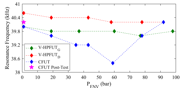
Fig. 8. Series resonance frequency as a function of P_{ENV} . There is an uncertainty of \pm 0.5 bar associated with the pressure measurements.
