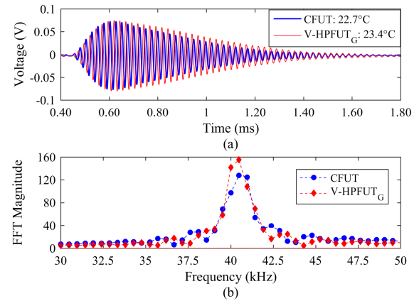
Fig. 7. (a) Pitch-catch ultrasound signals detected at 1 bar with a 20-60 kHz band-pass filter applied in signal processing; (b) FFTs of each response.
