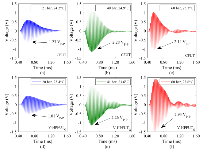
Fig. 9. Voltage responses and T_{ENV} for three magnitudes of P_{ENV} ( \pm 0.5 bar) for (a), (b), (c) the CFUT, and (d), (e), (f) V-HPFUT G as G, with V-HPFUT D as D in each case, and a 20-60 kHz band-pass filter applied in signal processing. The peak-to-peak voltages are also shown for each first response peak.
