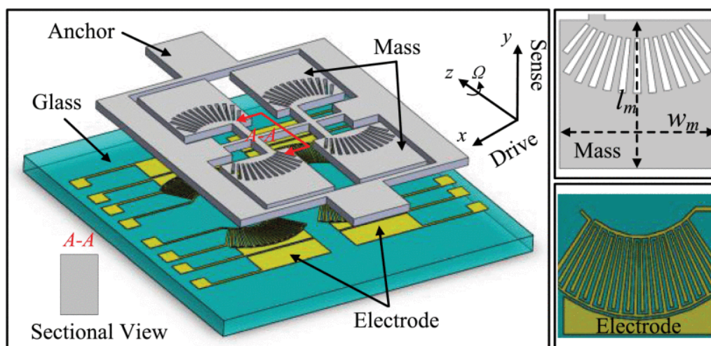
Butterfly micro-machined gyroscope fabricated by deep reactive ion etching (DRIE) processing (Vol. 19, No. 6, see page 2066).
