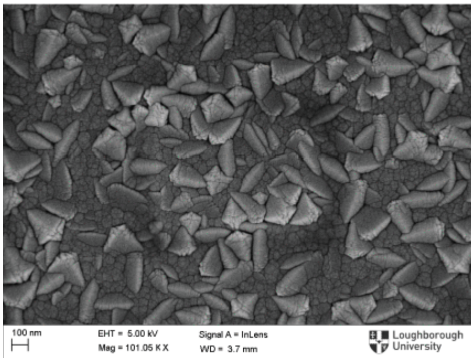
Humidity sensor structure with scanning electron microscope image of indium tin oxide structure sensor (Vol. 18, No. 18, see page 7359).
