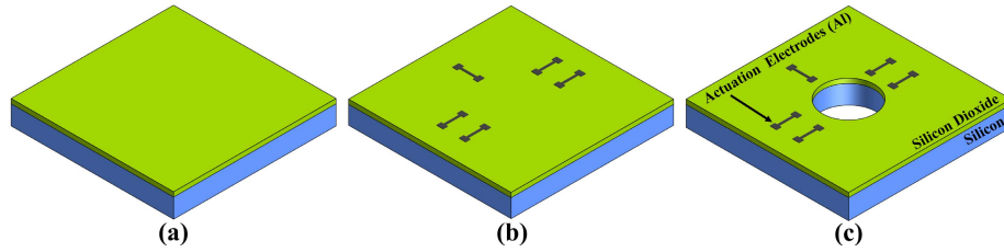
Fig. 1. Schematic diagram of the fabrication process for the desired substrate of graphene-PMMA resonator: (a) SiO 2 deposited, (b) Al sputtered and patterned, and (c) SiO 2 /Si etched and cavities created.
