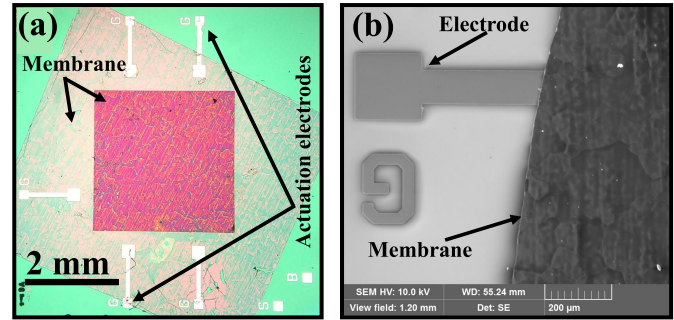
Fig. 3. (a) Optical micrograph of the suspended membrane over a square cavity. (b) SEM image of the membrane in contact with the actuation/tuning electrode.
