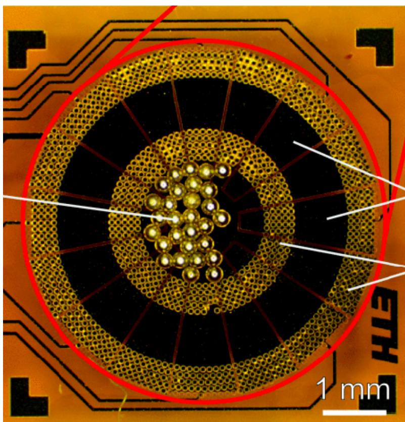
Macrograph of tilt sensor cavity before closure of cavity (see Vol. 17, No. 12, pp. 3640).
