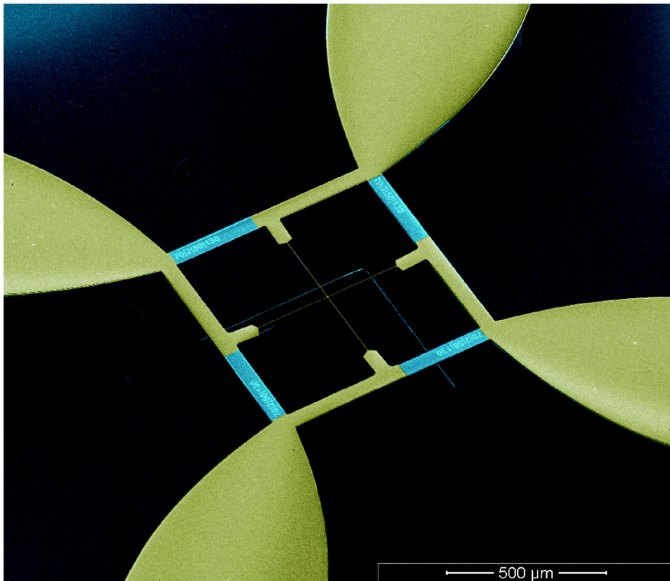
A 2D particle velocity sensor with minimal flow disturbance (see Vol. 16, No. 24, pp. 8707).
