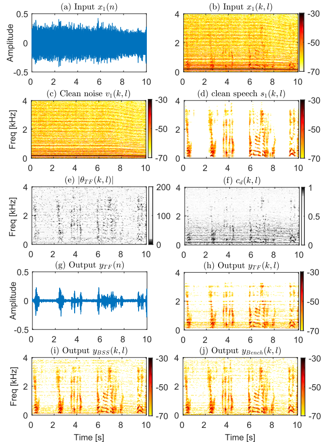
Fig. 3. Processing results with TF, BSS and Benchmark for a target sound with DOA 0^\circ and input SNR -10 dB. (a)-(b) Time-domain waveform and time-frequency spectrum of the input signal. (c)-(d): Time-frequency spectra of the clean ego-noise and clean speech signals. (e) Local DOA estimation results |\theta_{\text{TF}}(k, l)| . (f) Contribution measure to the target sound c_d(k, l, 0) . (g)-(h) Time-domain waveform and time-frequency spectrum of the TF output. (i)-(j) Time-frequency spectra of the BSS and Benchmark outputs. The output SNRs of TF, BSS and Benchmark are 13.9 dB, 14.4 dB and 14.5 dB, respectively.
