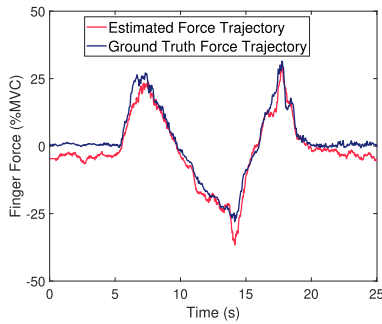
Fig. 6. Example waveforms of ground truth and estimated finger force trajectories (subject 2, session 1, middle finger, 2 nd trial of 1 DoF dataset). RMSE of the example trial was 3.56%MVC.
