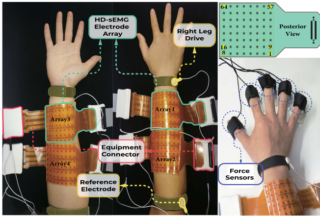
Fig. 1. Electrode Placement and Experiment Setup. We show photos of the same arm.
