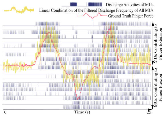
Fig. 7. Example MU discharge plot (subject 1, session 2, middle finger, 2 nd trial of 1 DoF dataset). The Pearson correlation coefficient of the presented trial is 0.8562.
