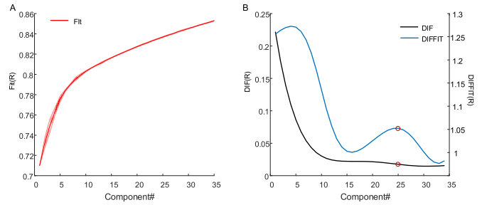
Fig. 5. The Fit, DIF, and DIFFIT curves in function of component R.
