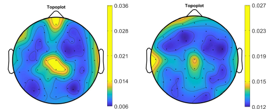
(a) SEED-IV
