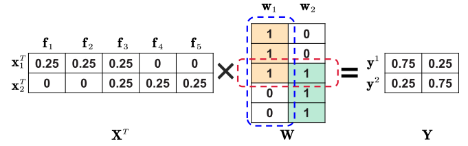
Fig. 1. An example to illustrate the two different types of features.
