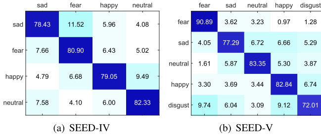
Fig. 4. The accuracies (%) of JCSFE represented by confusion matrices.
