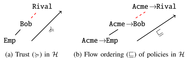
Fig. 1: Delegation loophole: By delegating to Rival, Bob effectively declassifies a label owned by Acme. Dashed lines indicate relationships influenced by Bob.
