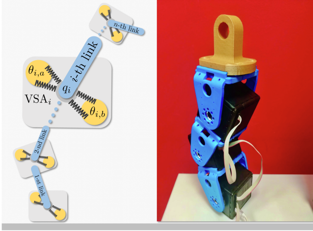
Fig. 1. Depiction of an articulated soft robot with n rigid links and n flexible joints driven by electromechanical VSA devices (left) and picture of the 3-degree-of-freedom hardware setup used to validate the proposed solution (right).
