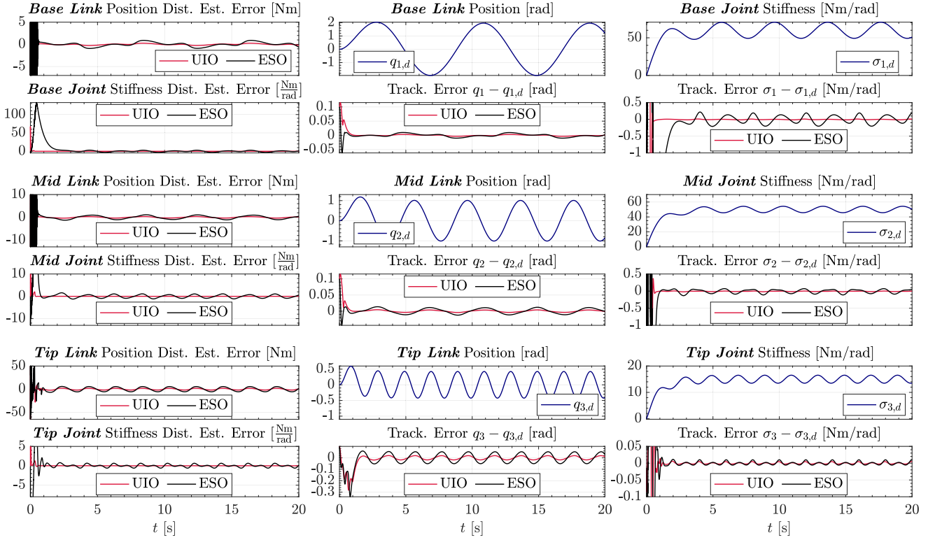
Fig. 3. Robustness to large uncertainty and comparison with ESO. Results from typical simulation runs with 100% deviation of system parameters from the nominal values, as well as a drastic simplification of the system model. Despite the large uncertainty, when the proposed DUJO-solution is used, the desired trajectories are accurately tracked as a result of fast and precise estimation of the disturbance perturbing the nominal system. The ESO-based solution under-performs especially when the disturbance signals are rapidly changing.
