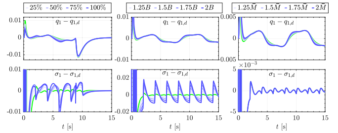
Fig. 2. Robustness to parametric (left), input matrix B (middle) and inertia matrix \bar{M} (right) uncertainties, ranging from 25% to 100% deviation from their nominal values. Green indicates the closed-loop behavior with nominal choices for parameters, B and \bar{M} . Position and stiffness tracking errors grow as uncertainty increases, yet, the closed-loop system performance does not deteriorate considerably. Tracking errors exist during time-varying references and are due to worse feedforward compensation, originating from larger parametric uncertainty and model simplification. Indeed, they nicely converge when references become still (last phase of left plots).
