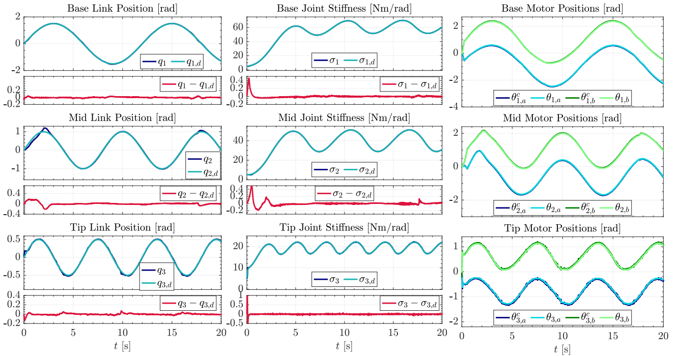
Fig. 4. Experimental validation. Results from testing with real ASR pictured in Fig. 1, when the task is to simultaneously track sinusoidal position and stiffness trajectories. The position and stiffness tracking errors are reported in red for each degree-of-freedom. Despite the drastically simplified robot model, upon which the estimator from Theorem 1 and the controller from Theorem 2 are derived, the proposed solution can robustly track the desired signals. Commanded \theta_{i,j}^c and executed \theta_{i,j} motor angles are shown and largely within the available range of the involved VSA devices.
