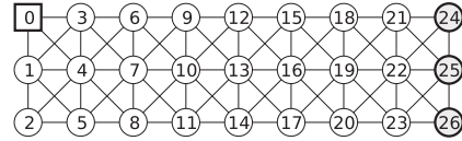
Fig. 2. A small scenario with V = \{0, \dots, 26\} , V_S = \{24, 25, 26\} . Here E_M = E_C and the edges are depicted by the lines between the vertices, W_{vw}^M = 1 , W_{vw}^C = 0 for all edges. The BS is the quadratic vertex 0, and the number of UAVs r is 3.
