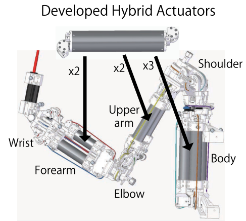
Fig. 3. Proposed robot configuration using developed hybrid actuators.
