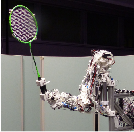
Fig. 1. Overview of the robot developed.
