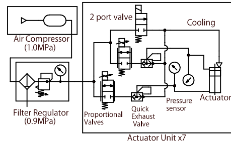
Fig. 6. Air circuit diagram.
