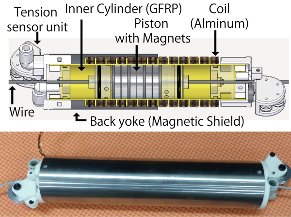
Fig. 2. Pneumatic-electric hybrid actuator and its mechanism.
