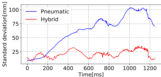
Fig. 11. Time series of the standard deviation at the racket head position in the precision experiment using the seven DoFs robot. Hybrid control is about 3.3 times as accurate as compared with only pneumatic control at around 1100 ms.
