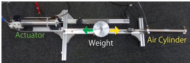
Fig. 8. Setup of the one-DoF experiment.
