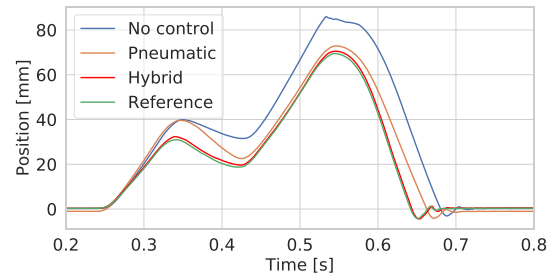
Fig. 9. Trajectories in the one-DoF experiment.
