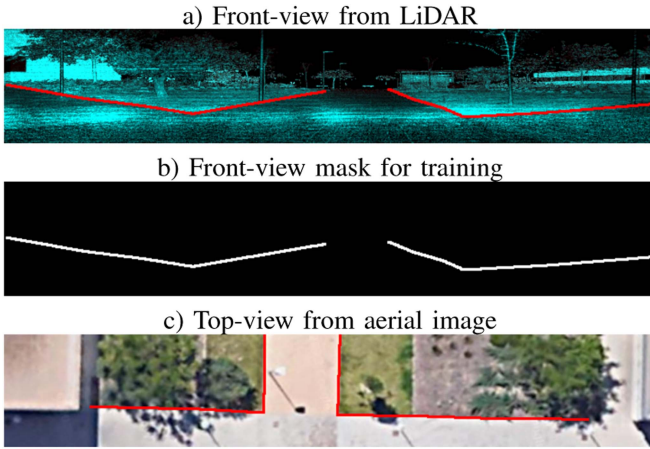
Fig. 2. Example of \mathcal{D}_i and \mathcal{L}_i : (a) Front-view from LiDAR information where the red line marks the ground boundaries ( \mathcal{D}_i ). (b) Front-view mask extracted from (a). (c) Top-view from the aerial image where the red line represents the exact boundaries shown in (a) and (b) ( \mathcal{L}_i ).
