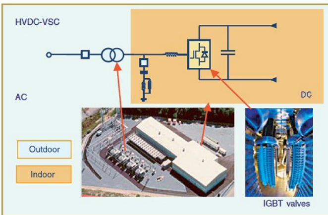
Fig. 3. HVDC with voltage source converters [7].
