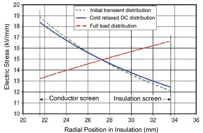
Fig. 14. Electric stress in DC cable insulation under different load conditions [23].
