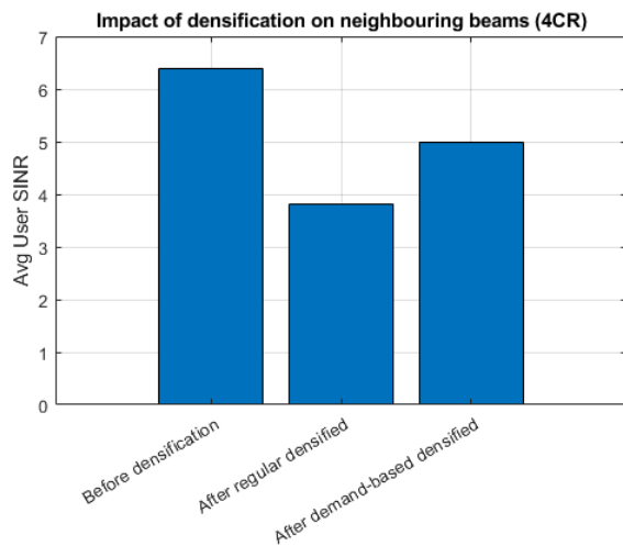
Fig. 39: Average user SINR on neighbouring beams
