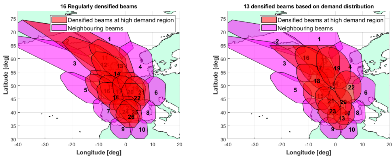
Fig. 5: Regular beam densification, where 4 beams are re- Fig. 6: Demand driven beam densification where the 4 beams placed by 16 beams are replaced by 13 beams
