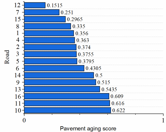
Fig. 7. Pavement aging index value for each road in the study area.
