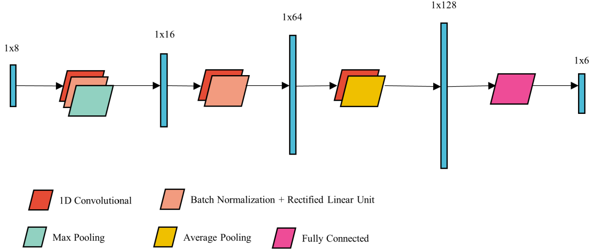
Fig. 8. The architecture of 1DCNN.
