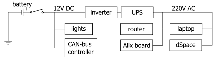
Fig. 2. Power supply setup for the system.
