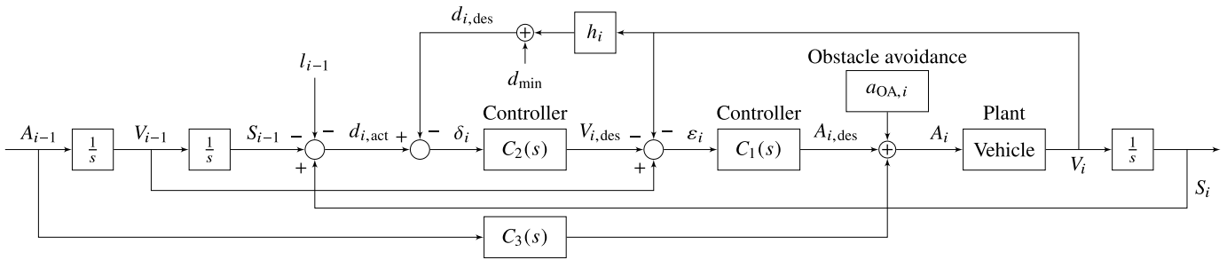
Fig. 5. Overview of the low-level control (LLC) system. C_1(s) is a speed controller, it keeps the speed of the previous vehicle and indirectly regulates the distance. C_2(s) regulates the distance to the vehicle in-front. C_3(s) manipulates the feed-forwarded acceleration A_{i-1} , from the preceding vehicle.
