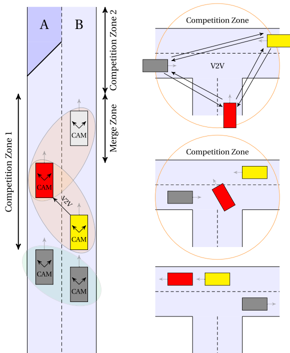
Fig. 1. The schematics of the two judged competition scenarios.
