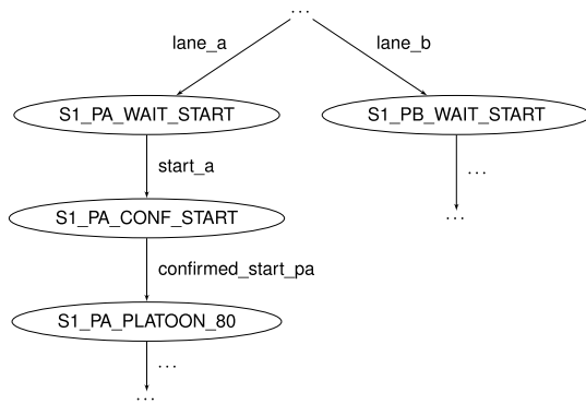
Fig. 7. Sample state transitions from [33].
