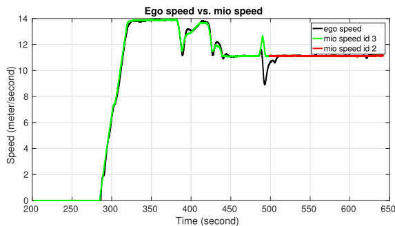
Fig. 10. CACC vehicle speeds during the merging heat.
