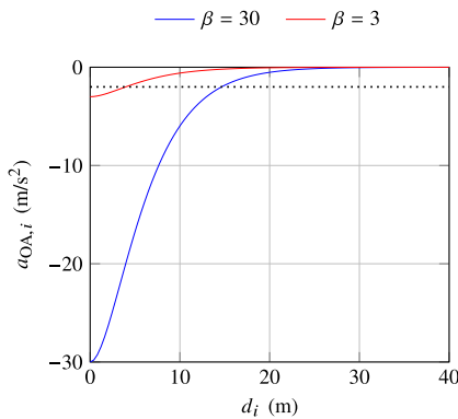
Fig. 6. Plot for OA with different \beta with black dotted line showing maximum (cut-off) deceleration of -2 \text{ m/s}^2 .
