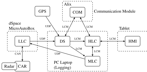
Fig. 4. Software system architecture.
