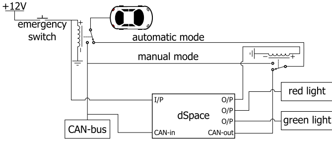
Fig. 3. CAN bus interface diagram.
