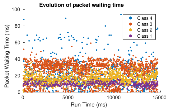
Fig. 16. SAPQ GCDC packet waiting times (high load).
