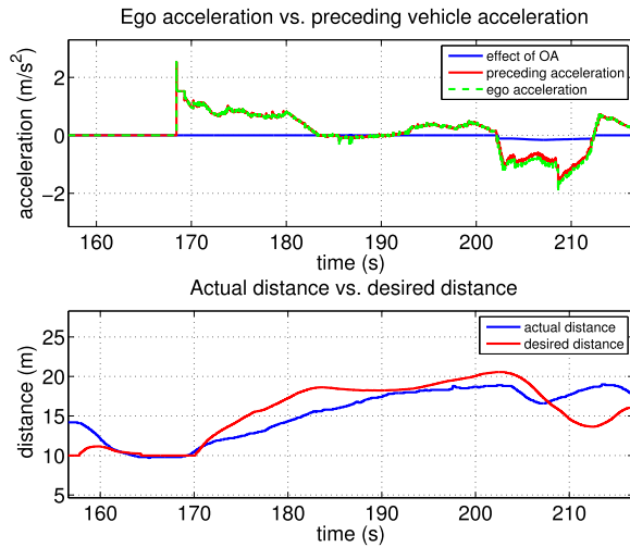
Fig. 13. CACC vehicle accelerations and distance with intended acceleration as input.
