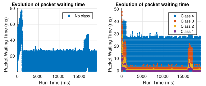
Fig. 15. FIFO (left) vs. SAPQ (right) packet waiting times (low load).
