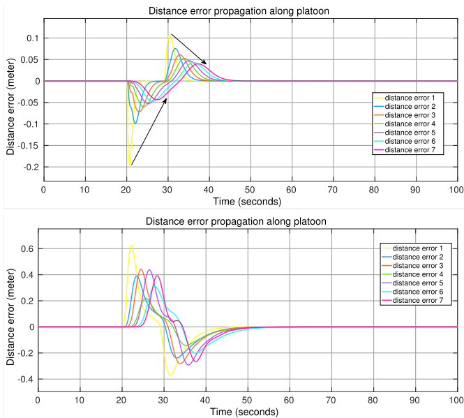
Fig. 9. Distance error propagation comparison to the SMA controller in a heterogeneous platoon simulation.
