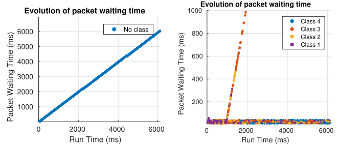
Fig. 14. FIFO (left) vs. SAPQ (right) packet waiting times (high load).
