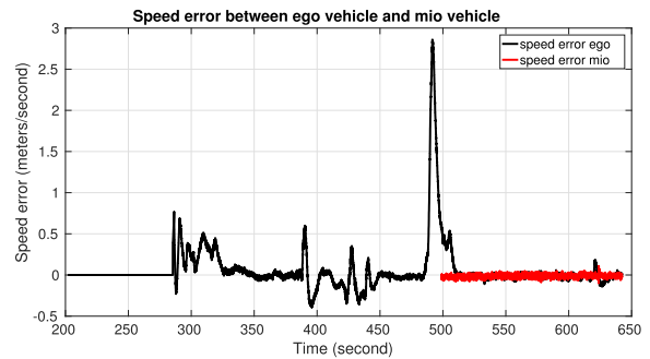
Fig. 12. Speed error for the speeds presented in Fig. 10.
