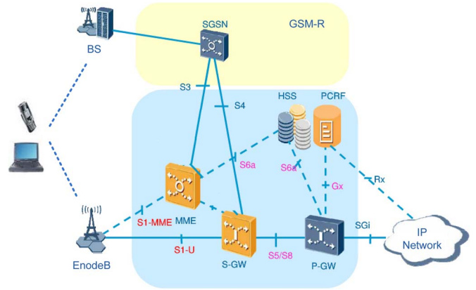
Fig. 12. Communication network architecture of LTE-R.
