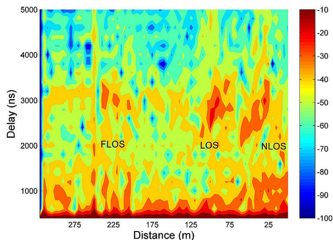
Fig. 8. Example plot of the PDP measured inside a subway tunnel in Madrid, Spain, from [50].
