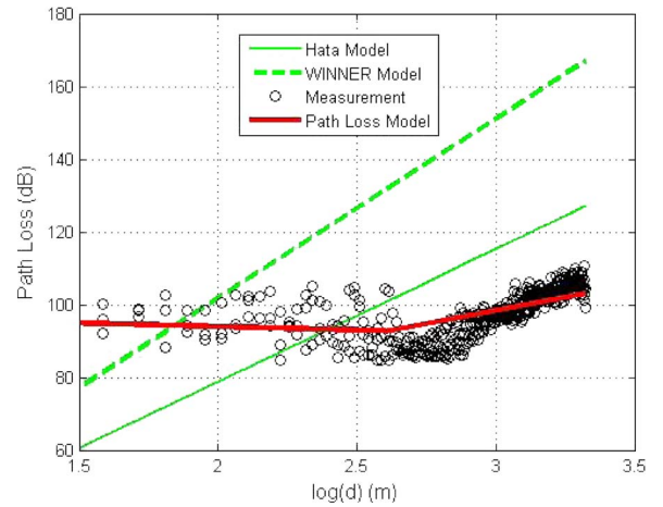
Fig. 5. Example plot of the path loss in the viaduct scenarios, from [38].
