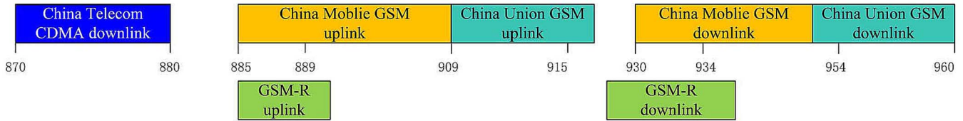
Fig. 2. Diagram of 800- to 900-MHz frequency allocation in China.
