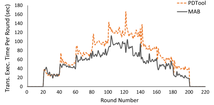
Fig. 10. MAB vs. PDTool transactional execution time convergence under CH-BenCHmark for dynamic workloads with different transaction levels.
