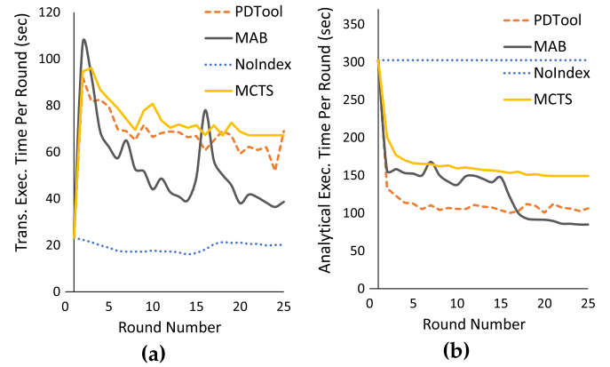
Fig. 5. MAB vs. PDTool versus MCTS convergence under CH-BenCHmark for static workloads with 3:1 TAR: (a) Transactional Execution cost, (b) Analytical Execution cost.
