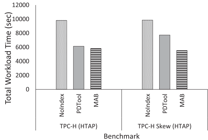
Fig. 6. MAB vs. PDTool vs. NoIndex total end-to-end workload time for static TPC-H and TPC-H skew HTAP workloads.
