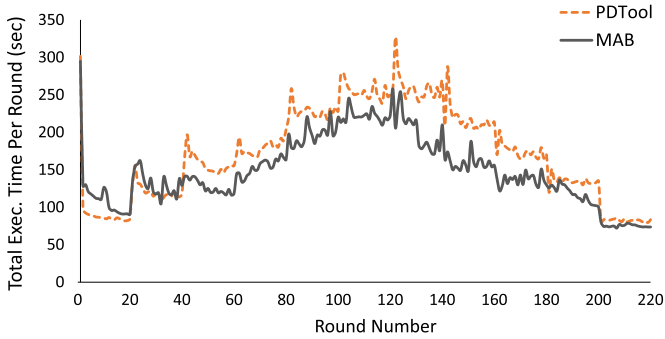
Fig. 8. MAB vs. PDTool total execution time convergence under CH-BenCHmark for dynamic workloads with different transaction levels.
