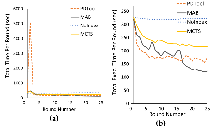
Fig. 4. MAB vs. PDTool versus MCTS convergence under CH-BenCHmark for static workloads with 3:1 TAR: (a) End-to-end workload time, (b) Total execution time.
