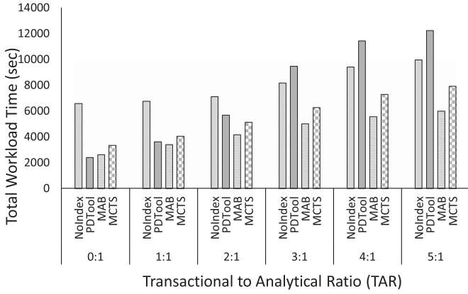
Fig. 3. MAB vs. PDTool vs. MCTS total workload time under CH-BenCHmark for static workloads with a range of different TARs.
