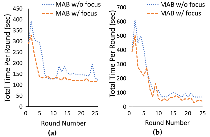
Fig. 14. MAB end-to-end workload time convergence with and without focus update for static analytical workloads: (a) TPC-H, (b) TPC-H Skew.
