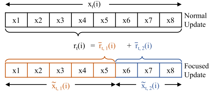
Fig. 2. Regular contextual updates versus focused update.
