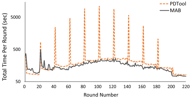
Fig. 7. MAB vs. PDTool total-workload time convergence under CH-BenCHmark for dynamic workloads with different transaction levels ( log y-axis ).
