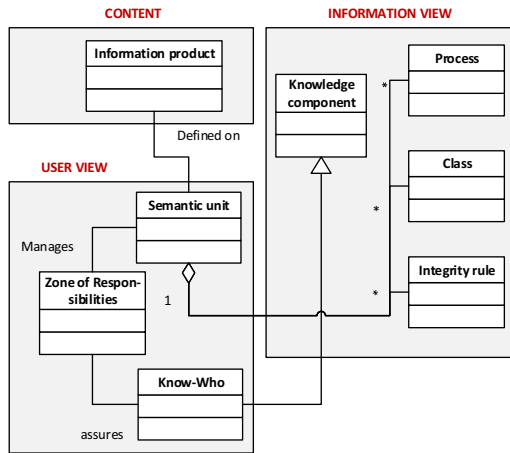
Figure 2. Excerpt of the meta-model related to user view
