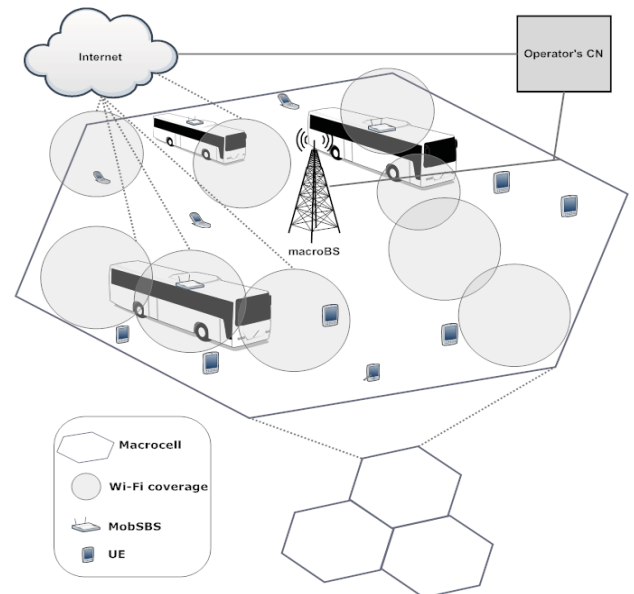
Fig. 1. Mobile small cells utilizing Wi-Fi Overview
