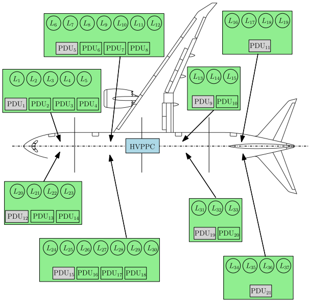
Fig. 4. Physical location of the devices of the considered subnetwork in Boeing 787. In the figure, the sketch of the aircraft is partially reproduced from [40].
