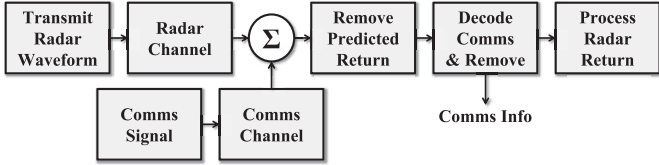
Fig. 6. Joint radar-communications system block diagram for SIC scenario. The radar and communications signals have two effective channels, but arrive converged at the joint receiver. The radar signal is predicted and removed, allowing a reduced rate communications user to operate. Assuming near perfect decoding of the communications user, the ideal signal can be reconstructed and subtracted from the original waveform, allowing for unimpeded radar access.
