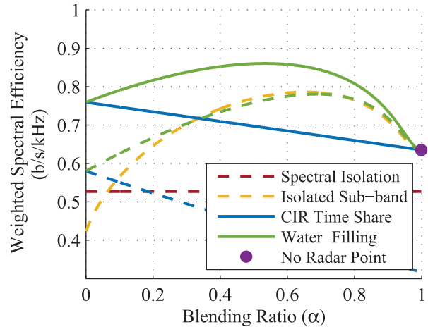
Fig. 13. Weighted spectral efficiency (measured here in bits per second per kilohertz) plots for joint radar-communications access, weighted for importance. In this example, we weighted the radar bits 3000x what the communications bits are worth. This may be true for certain military radar applications, and the weighting may be scenario dependent. With proper weighting, the maximum point of spectral efficiency has more meaning and utility.
