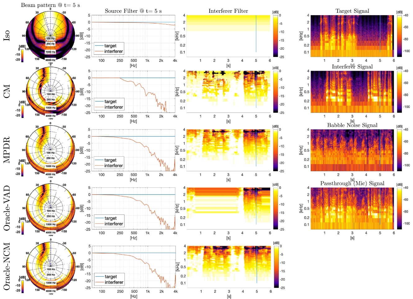
Fig. 3. The spatial, spectral and temporal visualisations of the filter gain (normalised by the transfer function of the reference microphone) for each beamformer in a trial with T_{60} = 0.2 s, C_{50} = 27.5 dB, SIR = -5 dB, SBNR = 15 dB and \Delta\varphi = 15^\circ using simulated RIR. The fourth column shows the spectrogram of the oracle signals for the anechoic target, anechoic interferer, reverberant babbles as well as the passthrough at the reference microphone. For each method (per row), the first three columns respectively show the instantaneous spatio-spectral beam pattern on the horizontal plane at time t = 5 s, the instantaneous filter response in the direction of target and interferer, and the spectrogram of the filter in the interferer's direction. The solid blue line on the plots in the third and fourth columns shows the time used for the instantaneous plots in the first and second columns and the dashed blue lines on the first column plots indicate the azimuth of the target and interferer.
