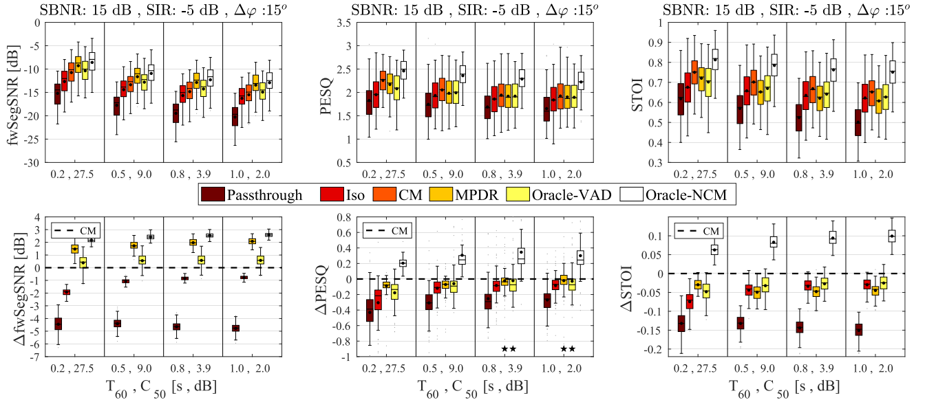
Fig. 2. Distribution of the evaluation metrics as absolute values (top row) and relative to CM (bottom row) for fixed SIR = -5 dB, SBNR = 15 dB, SSNR = 40 dB, \Delta\varphi = 15^\circ and varying reverberation using simulated RIRs.
