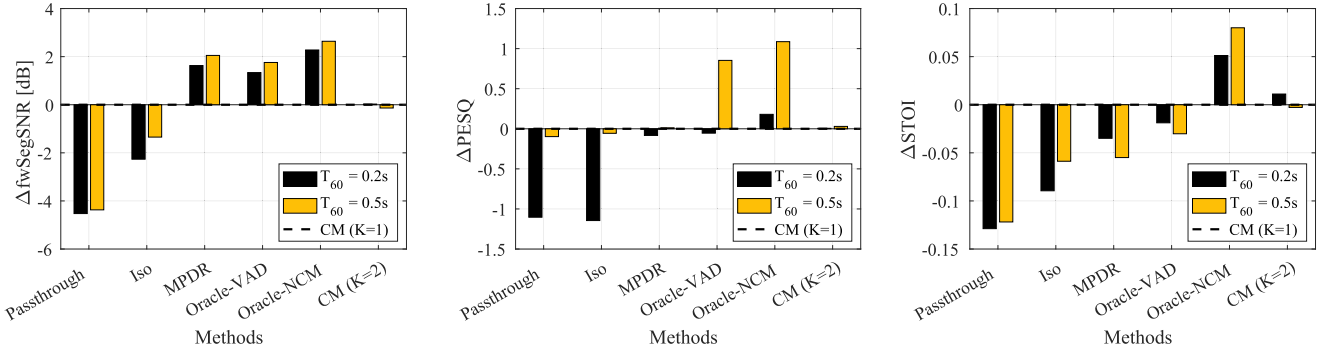
Fig. 4. The evaluation metrics of the methods relative to CM ( K = 1 ) in a trial with SIR = -5 dB, SBNR = 15 dB and \Delta\varphi = 15^\circ for varying T_{60} = [0.2\text{ s}, 0.5\text{ s}] using simulated RIR.
