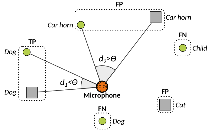
Fig. 4. Example reference and predicted sound events and locations. Circles denote reference sounds, rectangles denote system output. The dashed rectangles indicate associated predictions with references, and d_1, d_2 are the respective angular distances expressing localization error. The TP, FP, FN indicate how the respective predictions and references contribute to the true positive, false positive, and false negative count.
